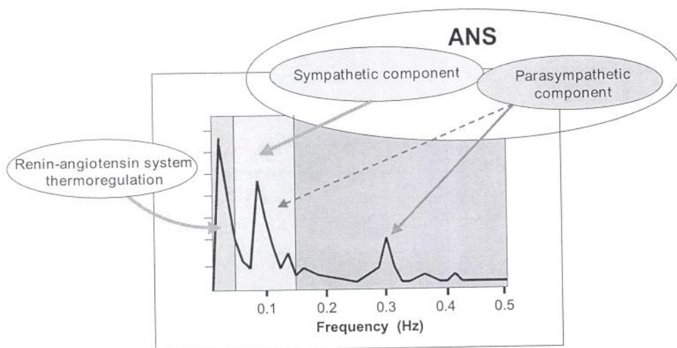
Figure 1. Physiological interpretation of spectral analysis R-R intervals results.
