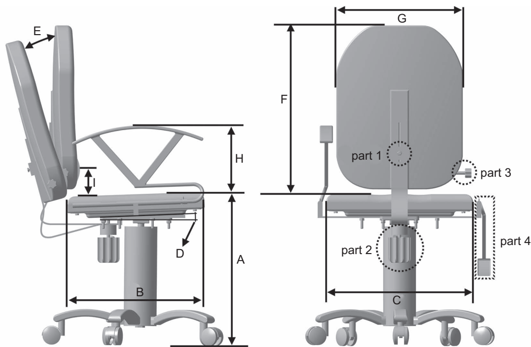
Figure 3. Dimensions of the new carpet-weaver’s chair. Notes. A, B, C, D, E, F, G, H, I = see Table 6.
